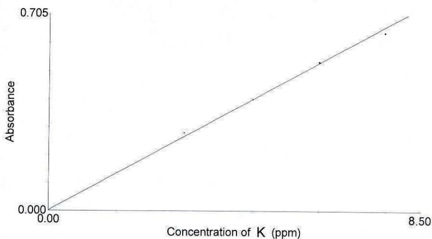
Figure 1. The standard curve of potassium ion.
